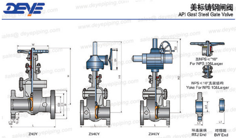
美标600Lb、900Lb铸钢闸阀 Class 600 & Class 900 Cast Steel Gate Valve
